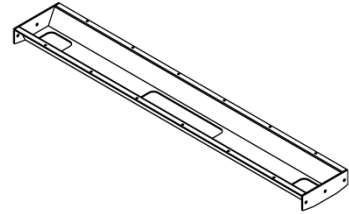
PLANNER STUDIO SUPPORT CHANNEL QTY. 1
